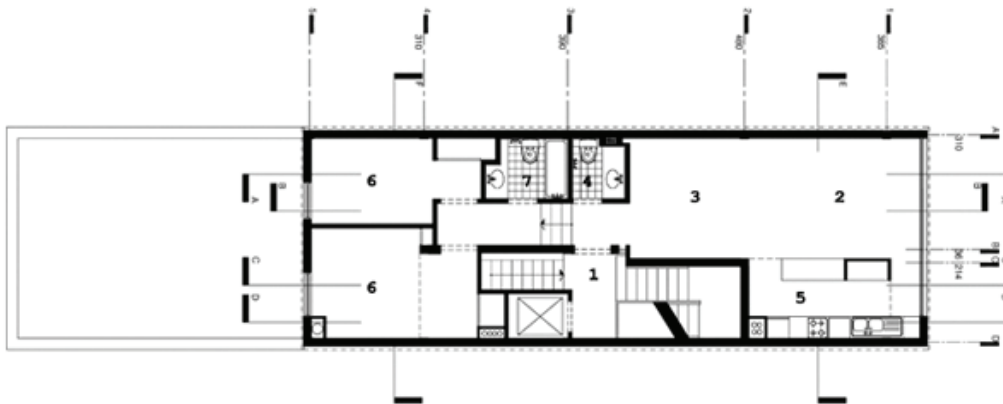
FIRST FLOOR PLAN Sc:1/100
