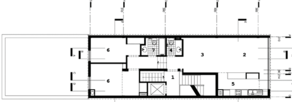
FIRST FLOOR PLAN Sc:1/100
